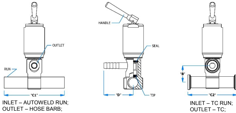
SANITARY ZERO STATIC TEE ANGLE SAMPLE VALVES - TOGGLE SAFETY HANDLE (Ø 0.370" INLET BORE SIZE)
